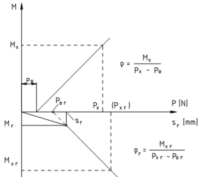
FIG. 19 MECHANICAL BRAKE
